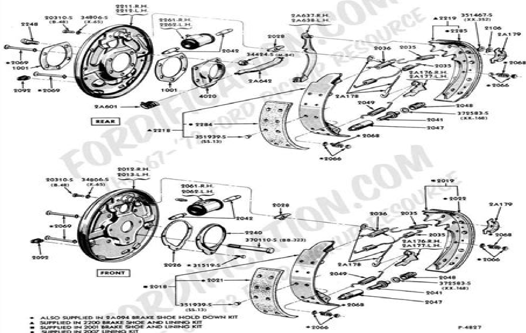
FRONT & REAR BRAKES - SELF ADJUSTING - TYPICAL 1964/72 E100/200, F100 (4 x 2) P100 1967 F100 (4 x 4), F250, F350/400
