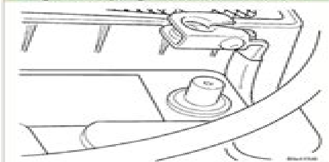
Fig. 10 Battery Negative Cable Remove/Install
