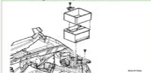
Fig. 11 Battery Remove/Install
