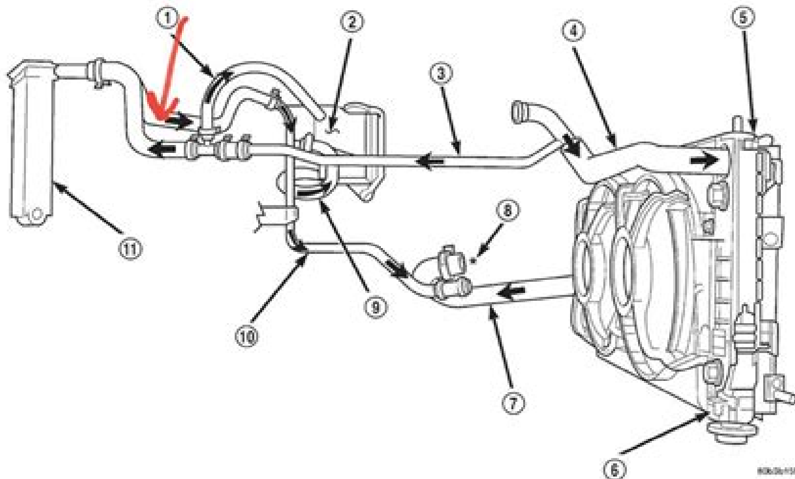
Fig. 1 COOLING SYSTEM FLOW
