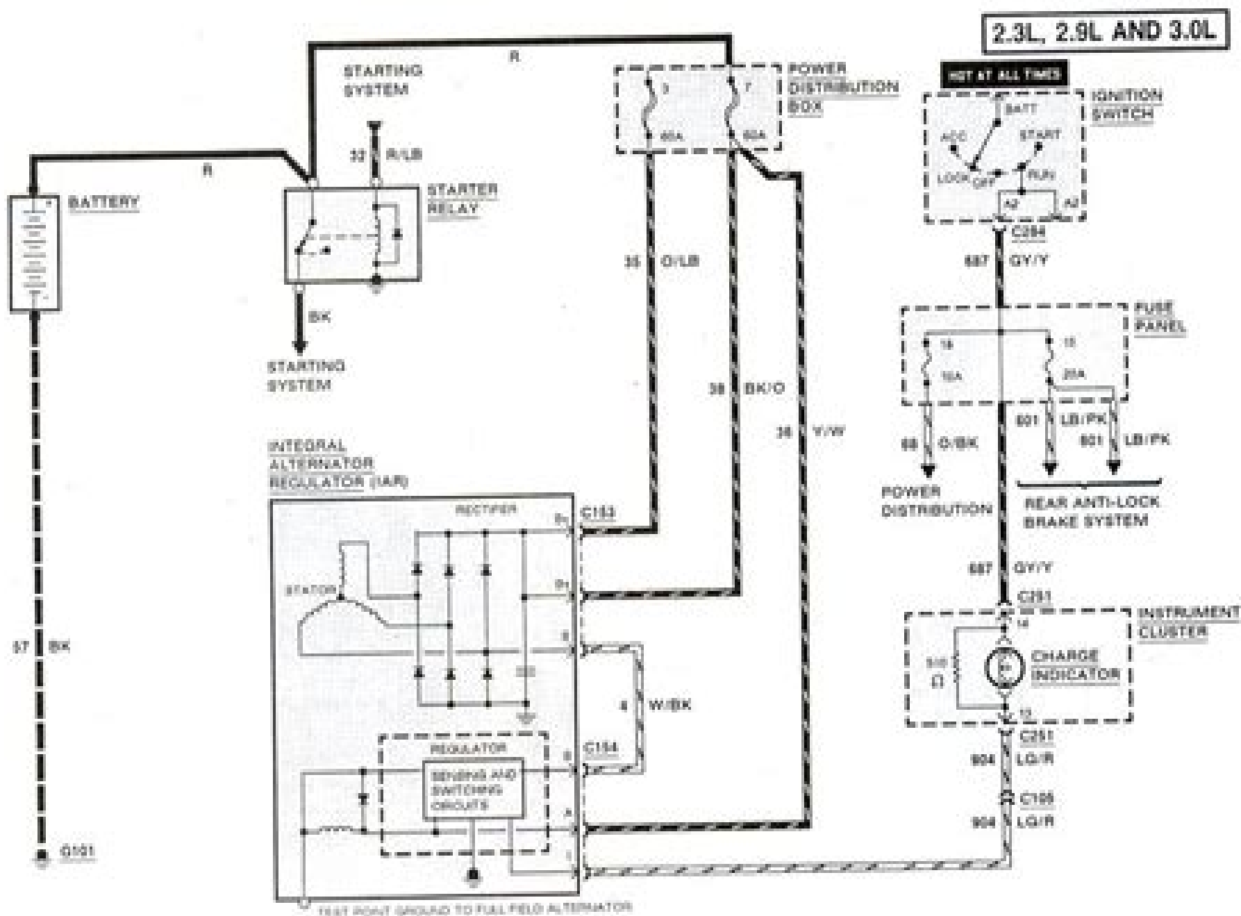
Charging system – late models (typical – 1991 shown) (part 2 of 2)
