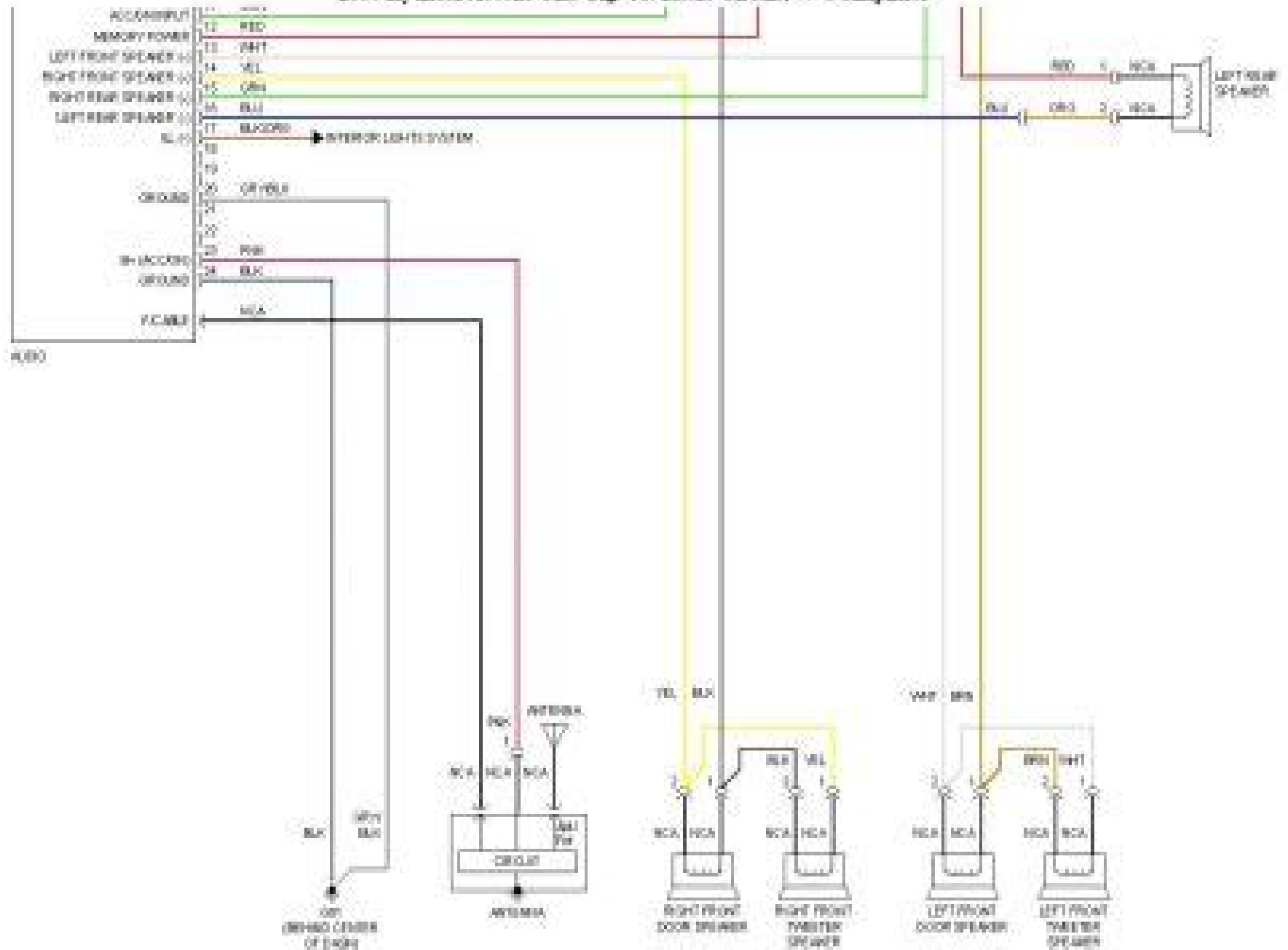
2000 Hyundai Accent GLS-Fig. 44: Radio Circuit, W/O Amplifier
