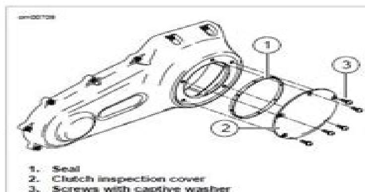
Figure 1-11. Clutch Cover
