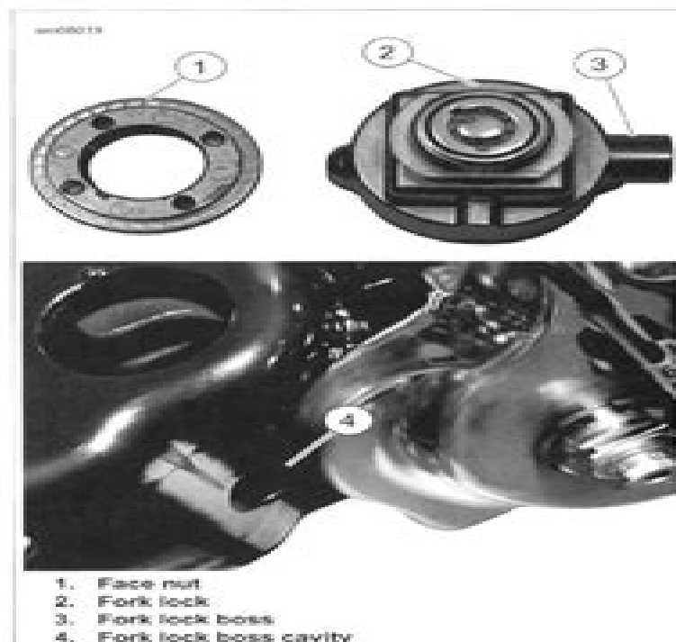
Figure 2-166. Fork Lock
