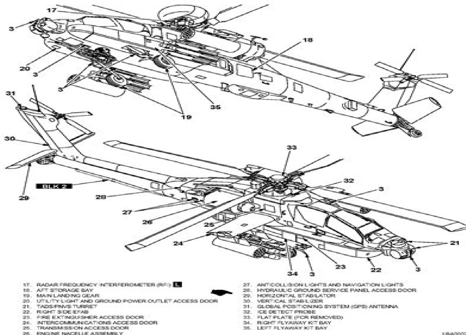
Figure 2-1. General Arrangement (Sheet 2 of 2)
