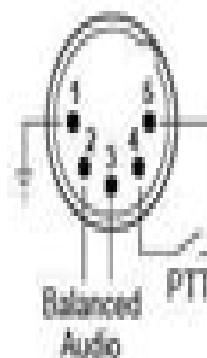
C 0379 5 Pin XLR Wiring Diagram
