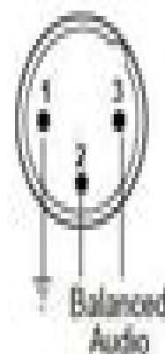
C 0377 3 Pin XLR Wiring Diagram
