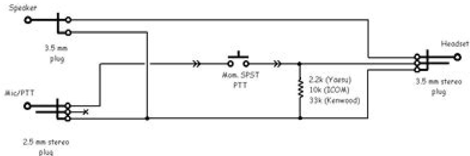
PTT for common VHF/UHF HTs
