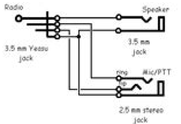
Yaesu CT-44 Adapter
