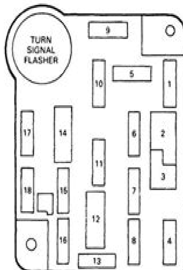
FUSE PANEL DIAGRAM - E-150 - E-350
