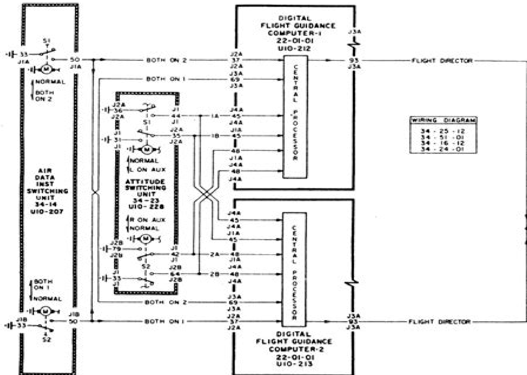
Figure 2-21. Wiring diagram.
