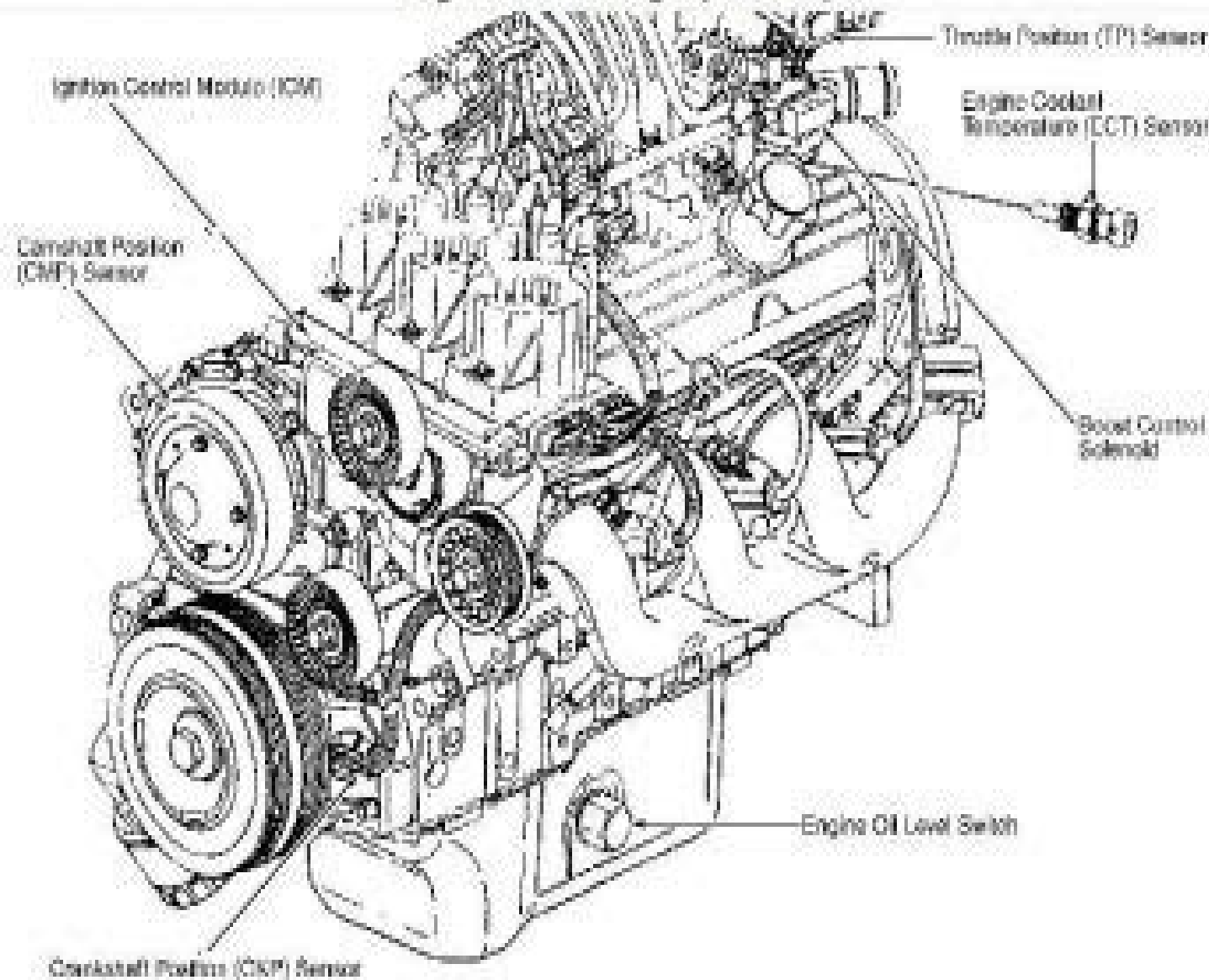
Fig. 5: Left Side Of Engine (3.8L VIN 1)
