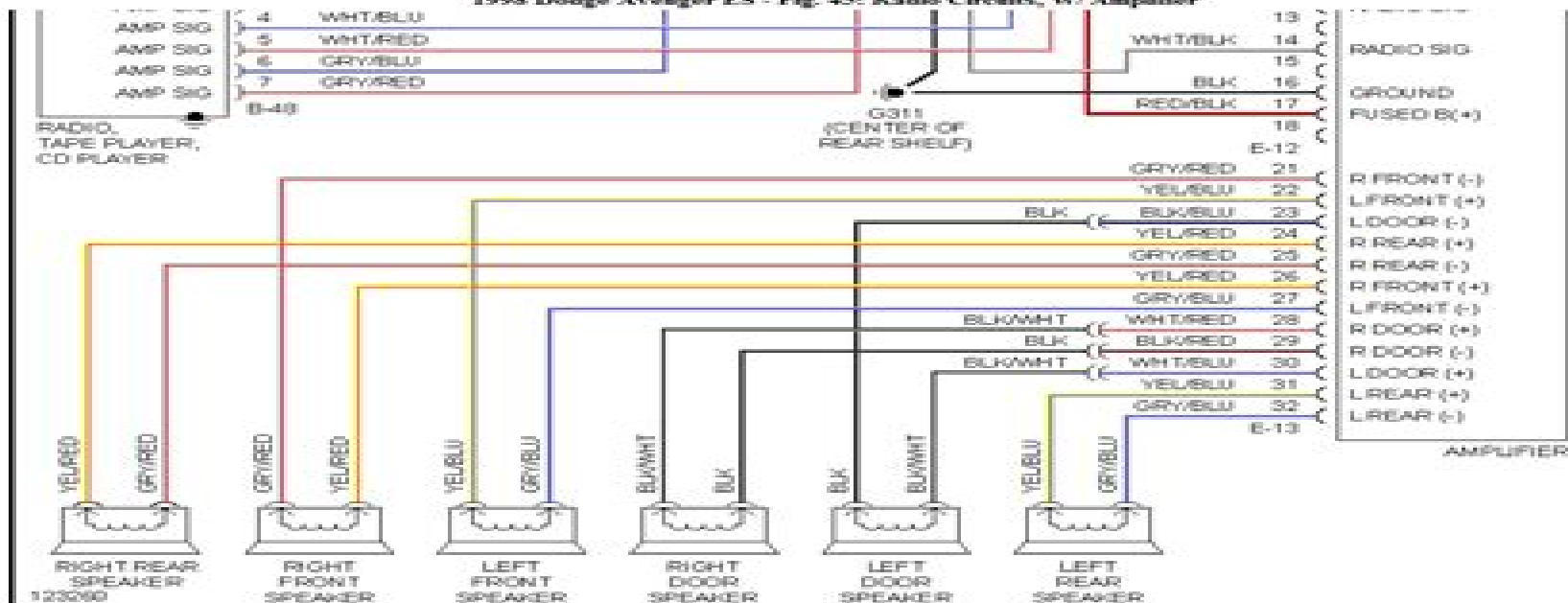
1998 Dodge Avenge ES - Fig. 45: Radio Circuits, W/ Amplifier
