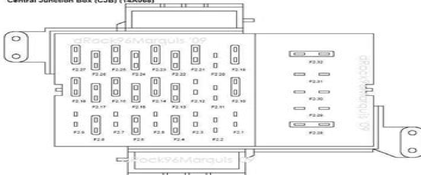
Central Junction Box (CJB) (14A068)
