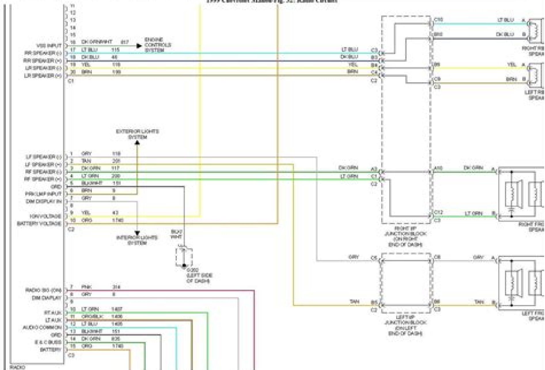
1999 Chevrolet Malibu—Fig. 32: Radio Circuits
