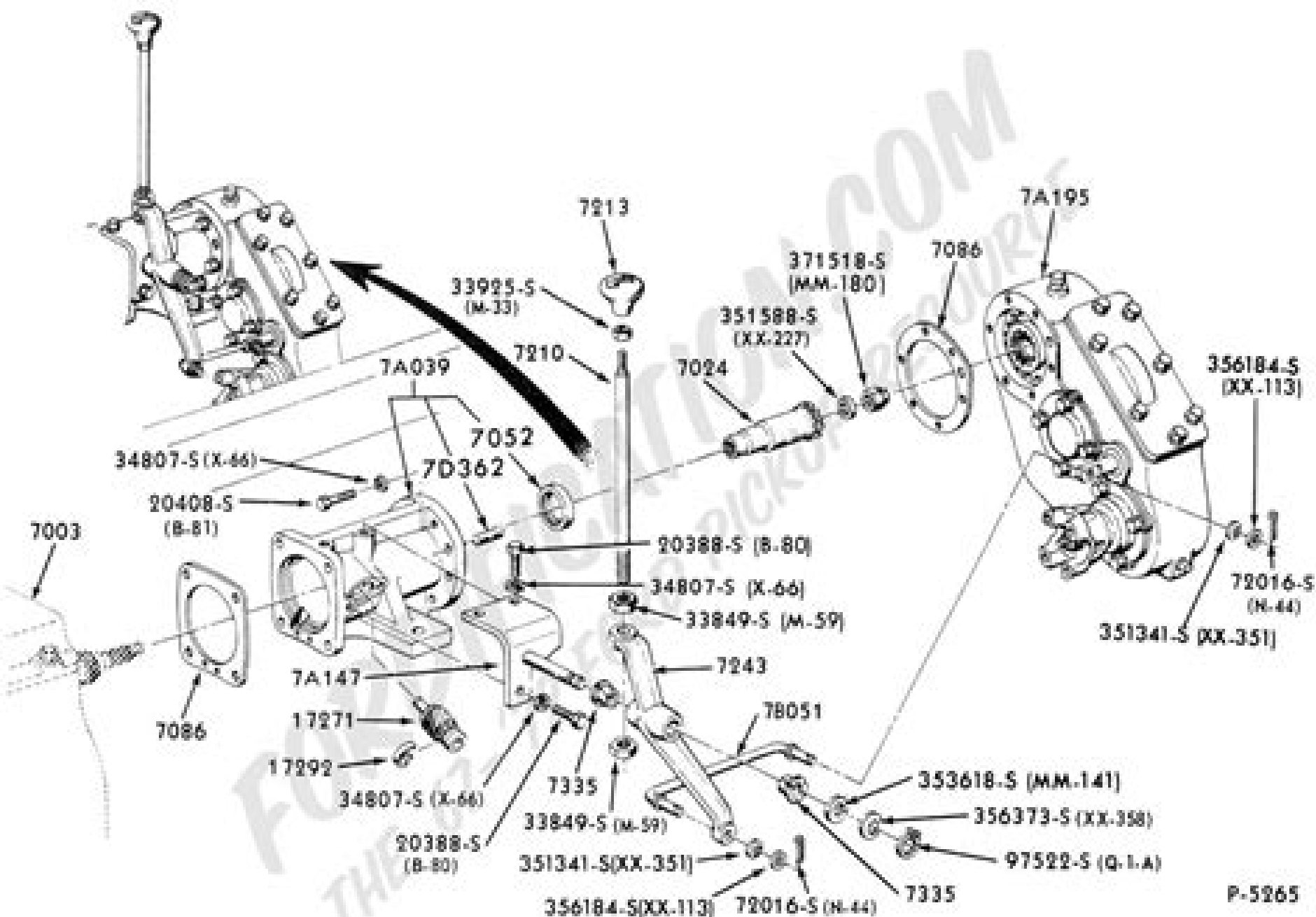
TRANSFER CASE SHIFT CONTROL & SUPPORTS-FOUR WHEEL DRIVE 1966/72 F100
