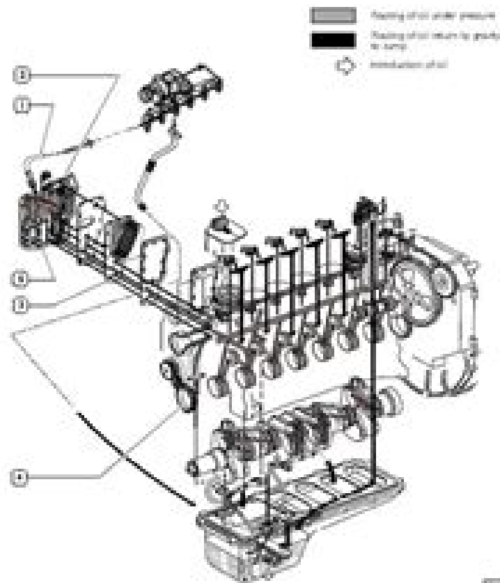
LUBRICATION SYSTEM LAYOUT (as an engine)
