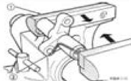
Fig. 95 Compressing Timing Belt Tensioner
