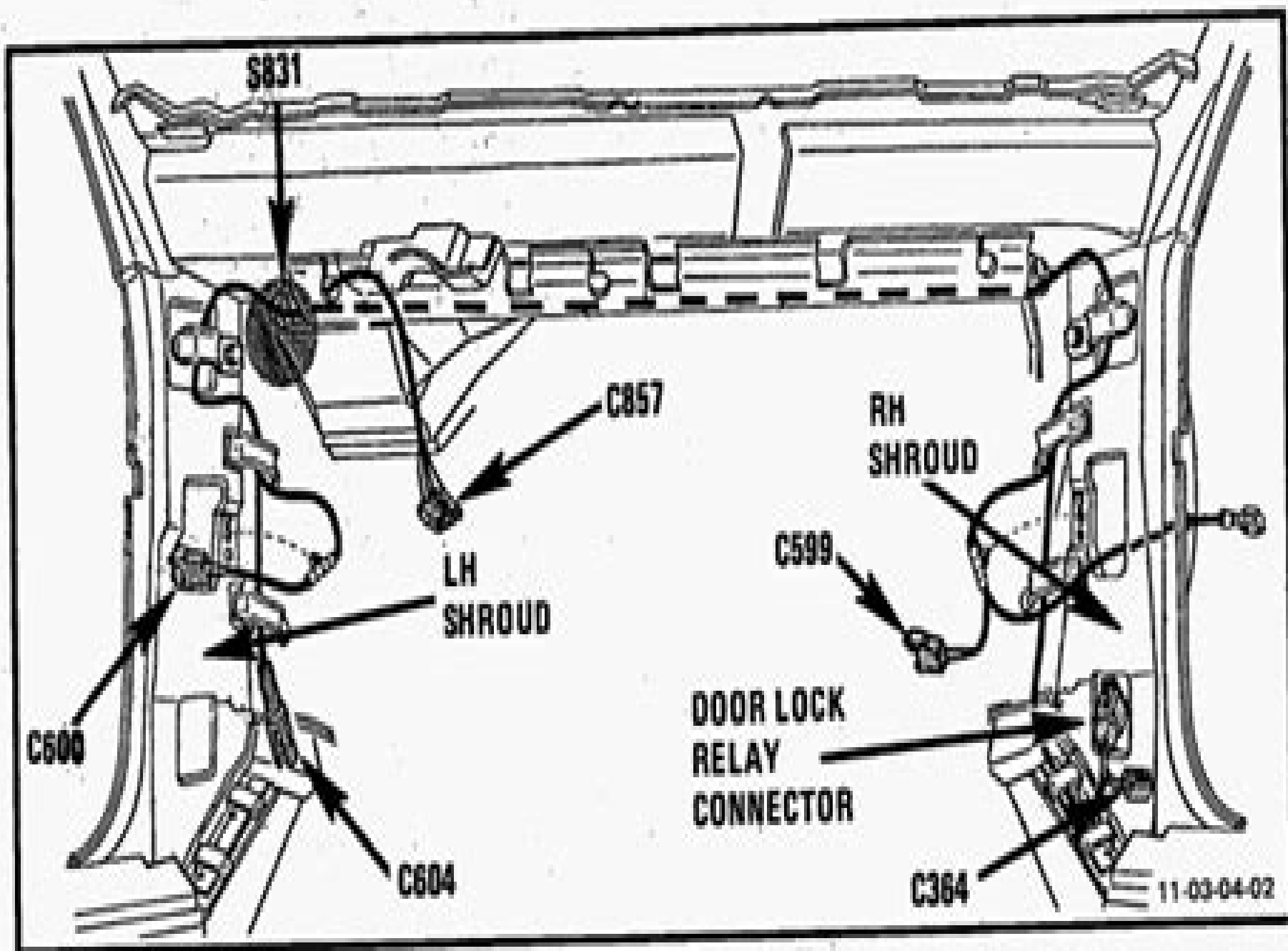
Figure B - Behind I/P, Cross Car Harness
