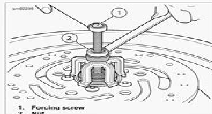
Figure 2-16. Remove Bearing
