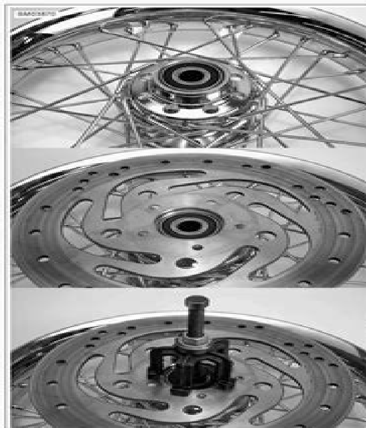
Figure 2-15. Brake Disk as Puller Aid
