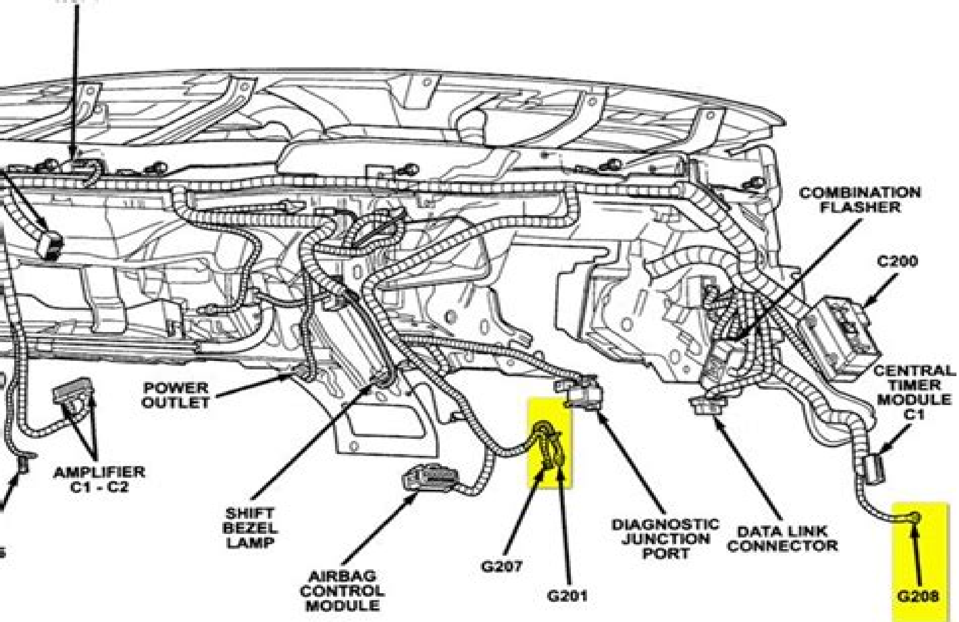
Fig. 32 INSTRUMENT PANEL CONNECTORS
