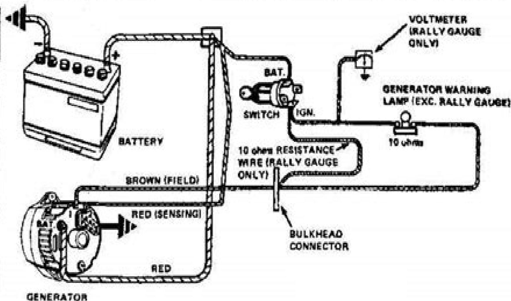
Fig. 6D-3C-Charging Circuit - Si System
