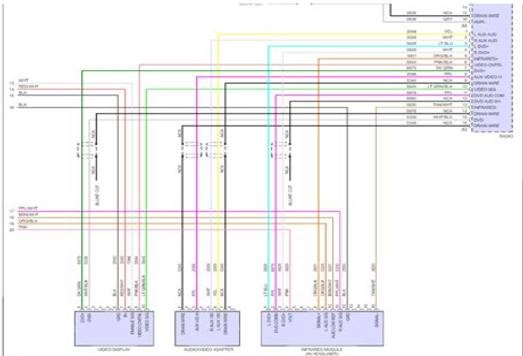
Fig 3: Radio Circuit, W/ Y91 & W/ UQA (3 of 3)
