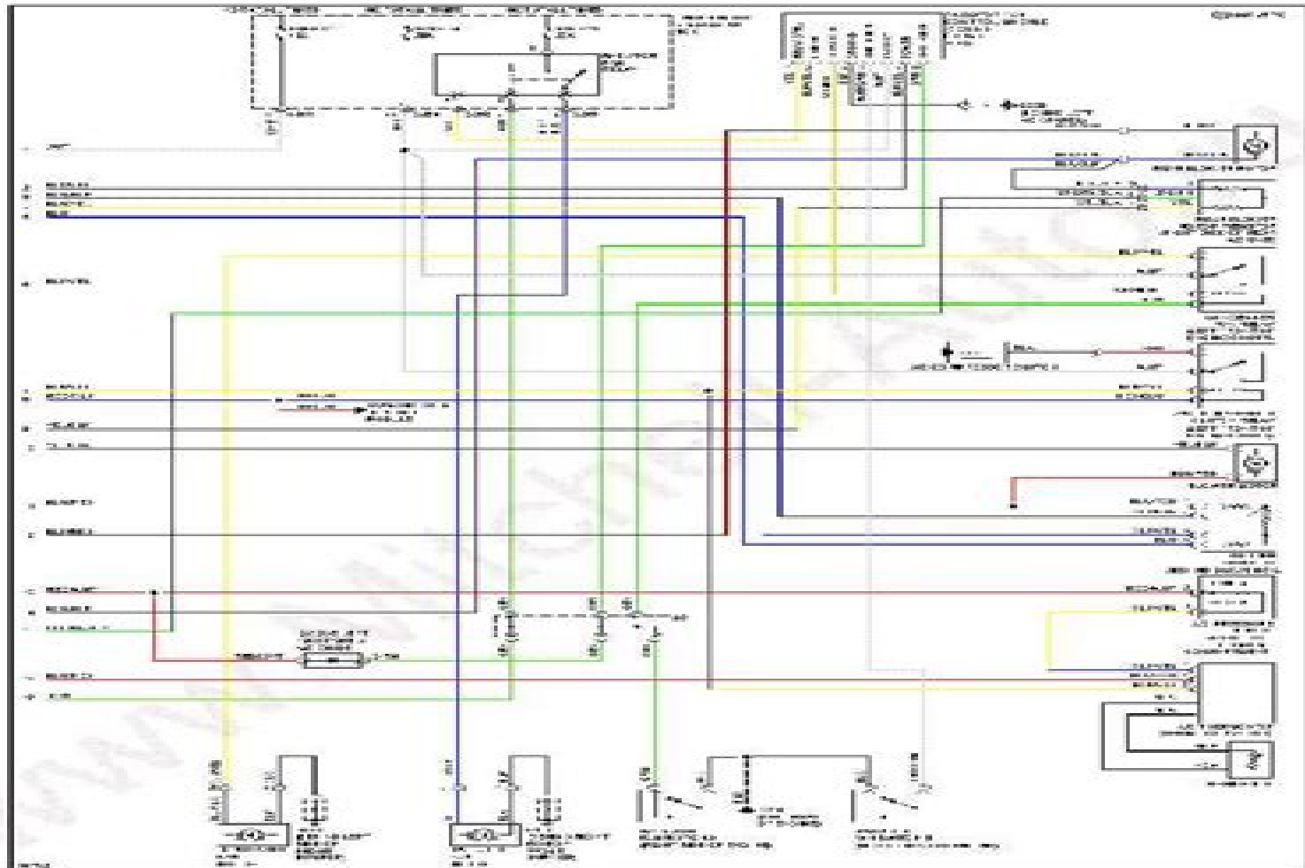
Fig. 2: Air Conditioning Circuits (2 of 2)
