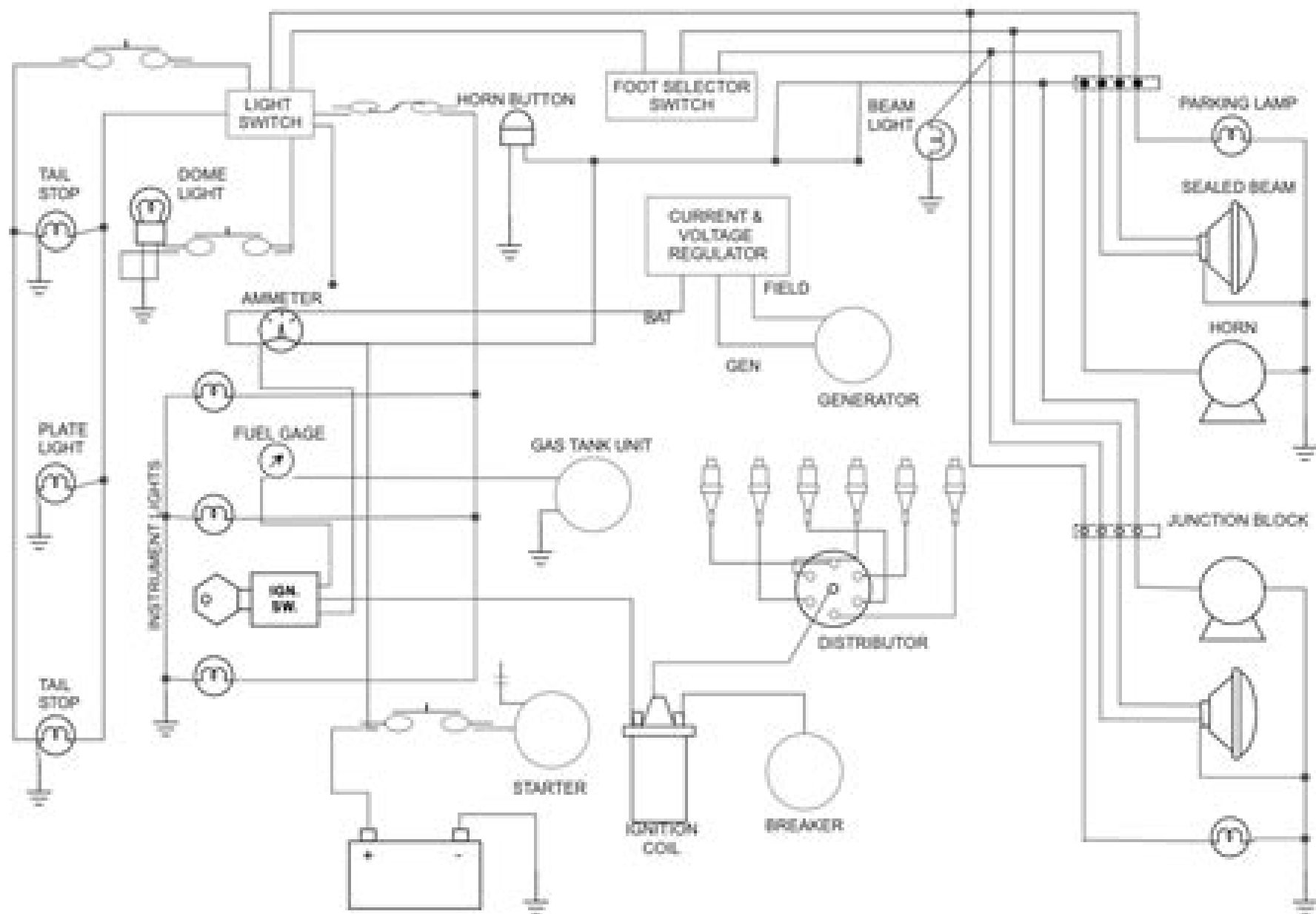
WIRING DIAGRAM AUTO ELECTRICAL WIRING DIAGRAM
