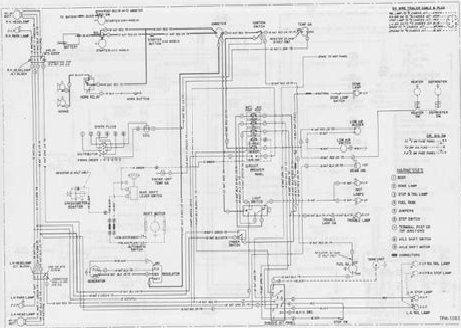
Figure 2—Wiring Diagram—Early Gasoline Models—Conventional Series 740-90 and up, and all C.O.E. Series
