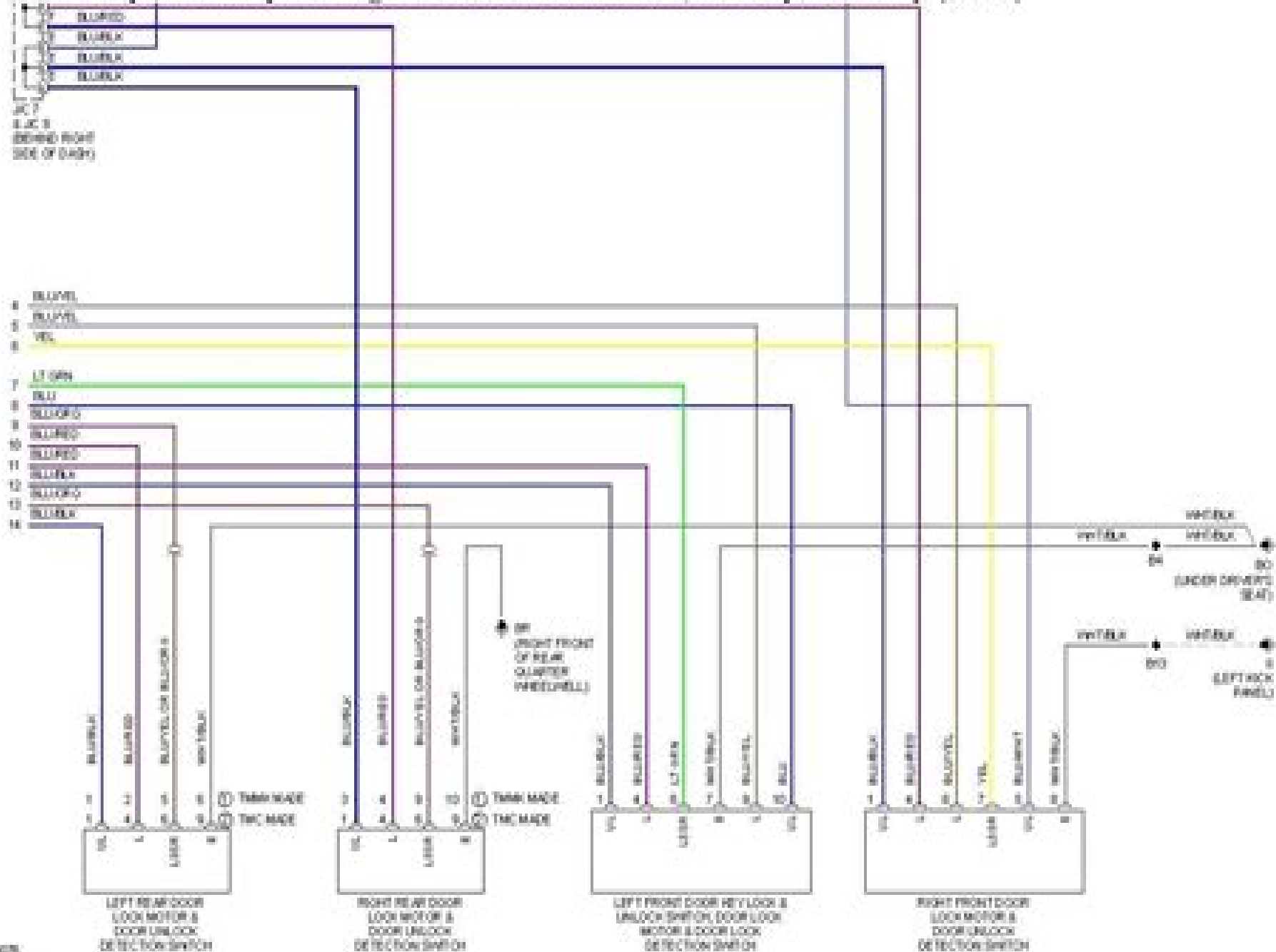
2002 Toyota Camry LE-Fig. 57: Door Lock Circuit, W/ Keyless Entry (2 of 2)
