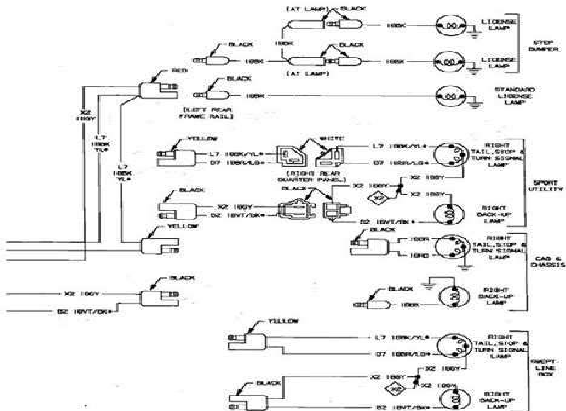
Fig. 38 Rear Lighting System Wiring Circuit (Part 2 of 2)
