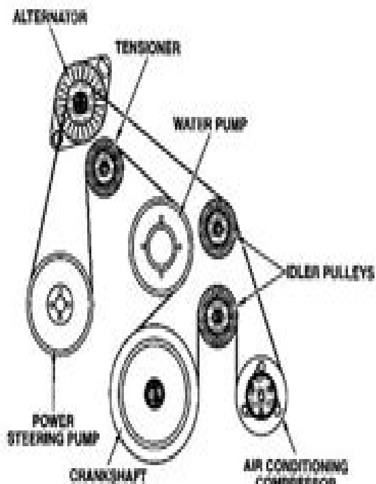
Drive belt installation schematics.
