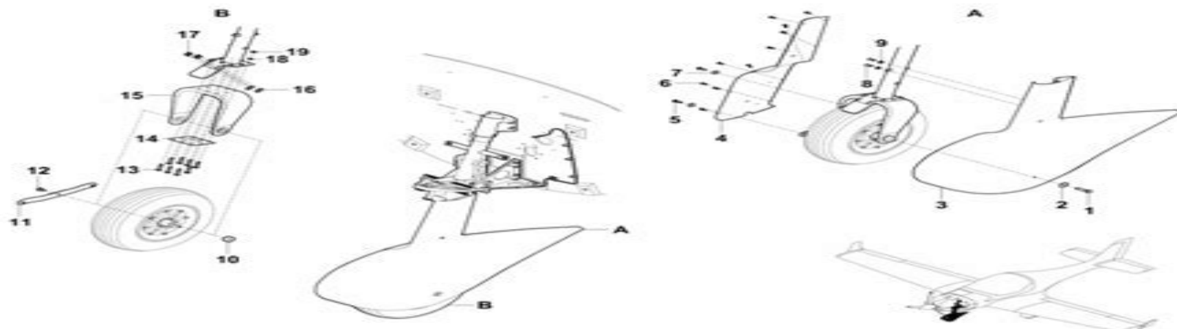
Figure 32-20-01 Nose Gear LSA
