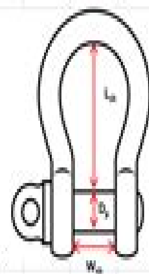
Fig 2: Shackle Geometry (For illustration purpose only)
