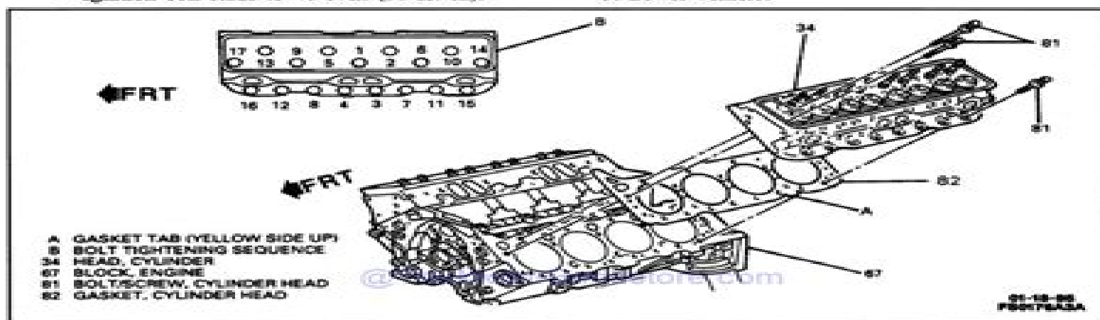
Figure 20 - Cylinder Head
