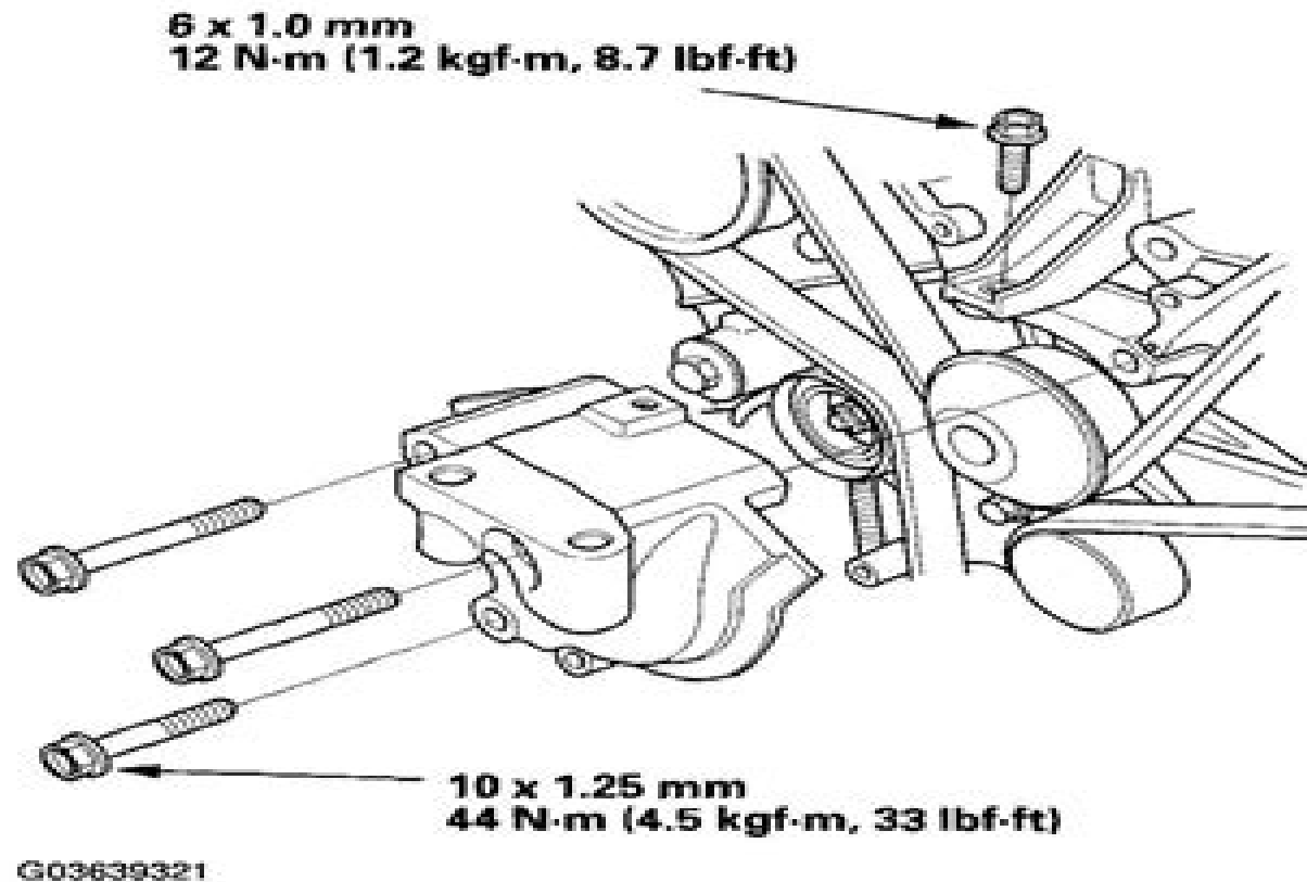
Fig. 43: Installing Lower Half Of Side Engine Mount Bracket Courtesy of AMERICAN HONDA MOTOR CO., INC.
