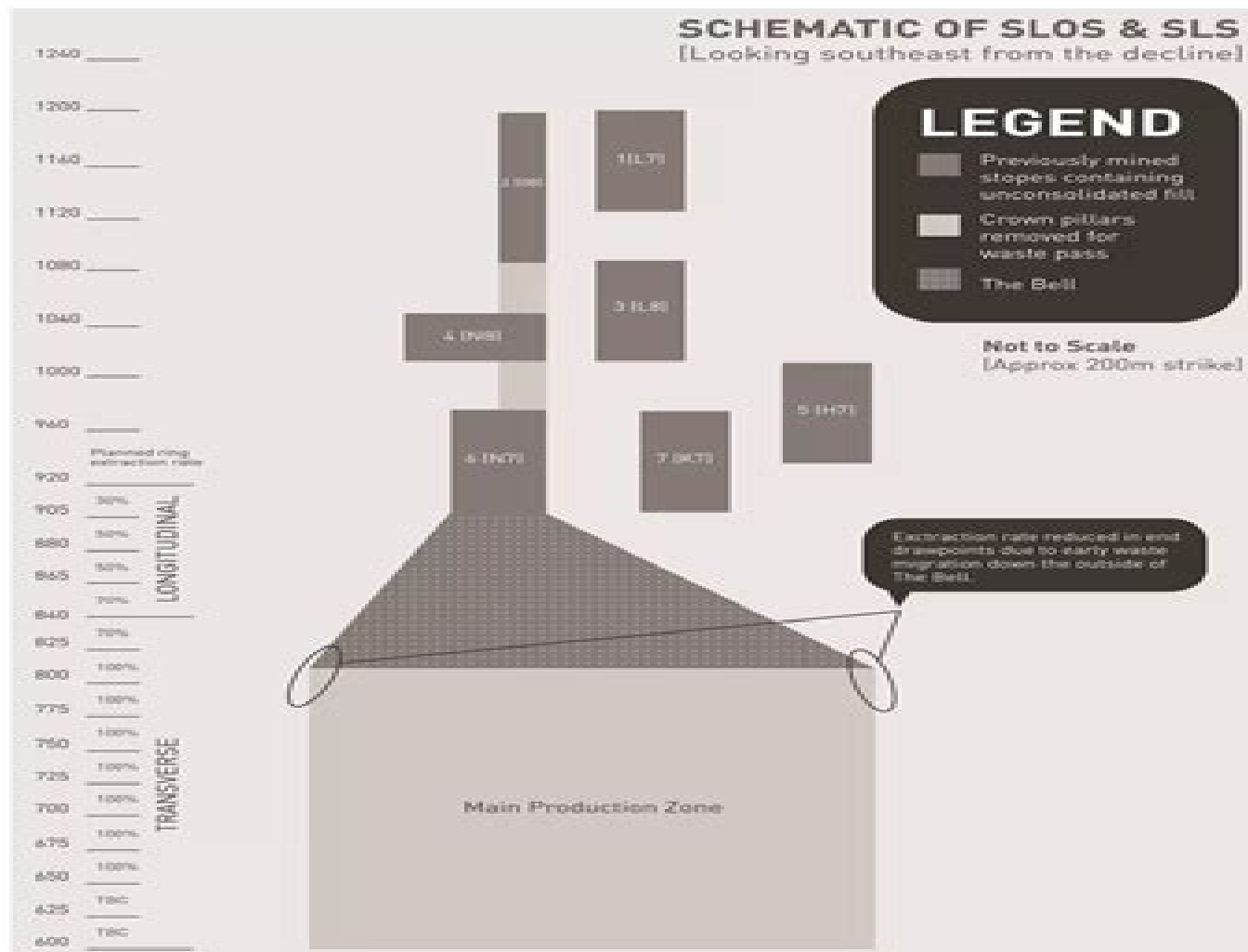
FIG 3 – A schematic section through the Mt Wright orebody looking south-east (from the decline).
