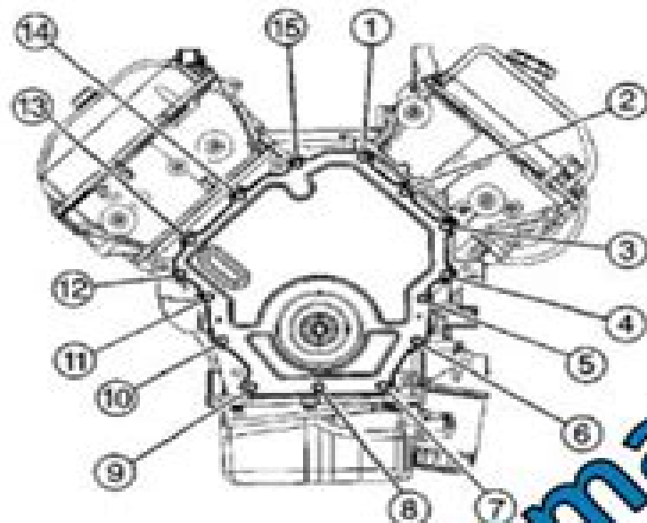
Fig. 72: Identifying Engine Front Cover Bolts Tightening Sequence Courtesy of GENERAL MOTORS CORP.
