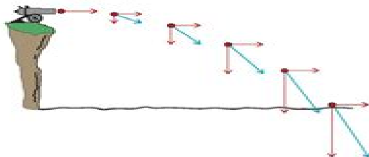
Figure 1.3 Velocity of a projectile is the sum of the vertical and horizontal velocities
