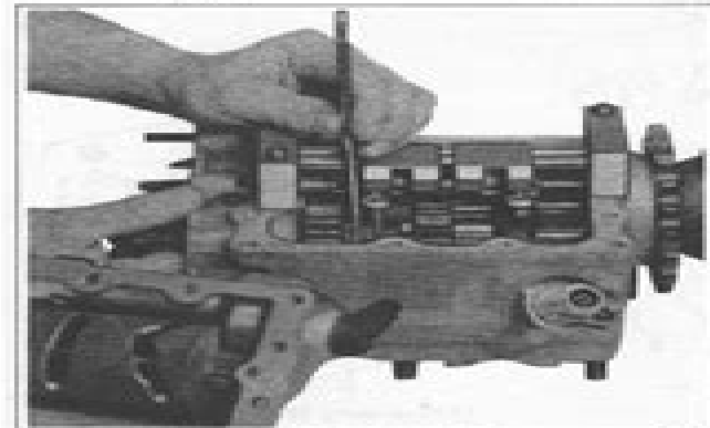
Figure 4-18. Checking Shifter Clutch Clearance — Early 1979 and Earlier
