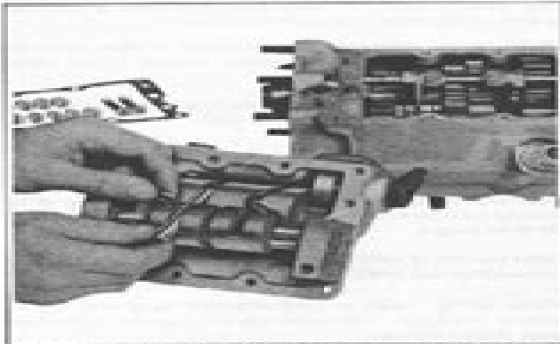
Figure 4-17. Adjusting Shifter Gauge — Early 1979 and Earlier
