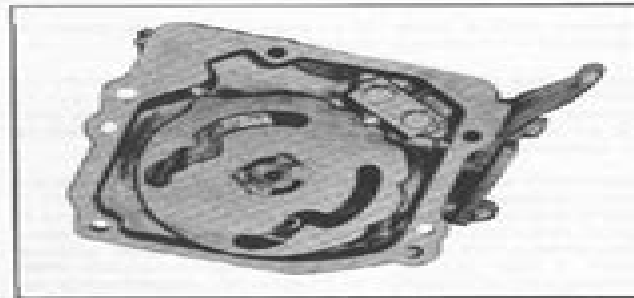
Figure 4-18A. Shifter Cam in Neutral Position — Late 1979 and Later
