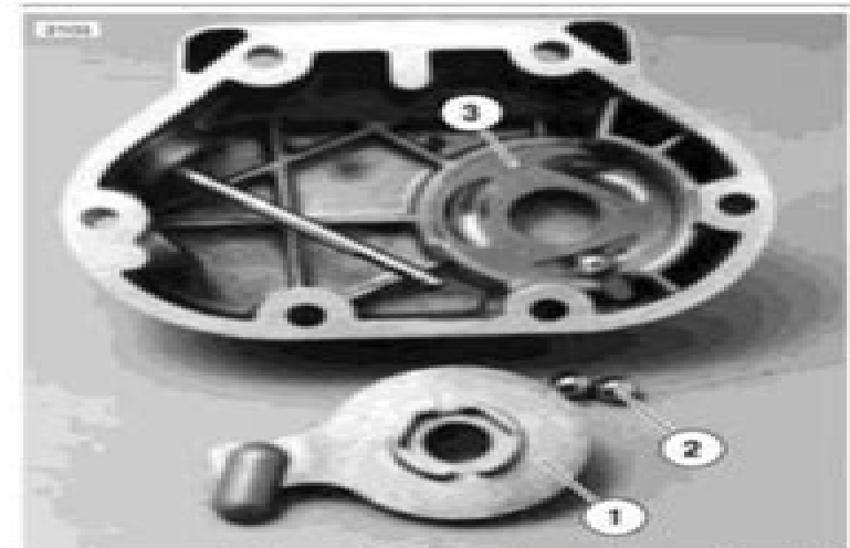
Figure 7-16. Coupling and Ramp Assembly 1. Inner ramp 2. Balls (3) 3. Outer ramp
