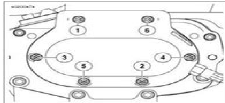
Figure 7-14. Cover Screws
