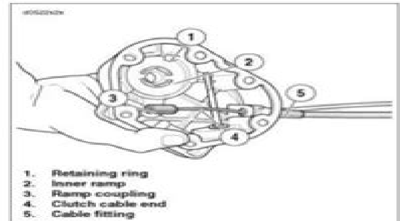
Figure 7-15. Clutch Cable Connection
