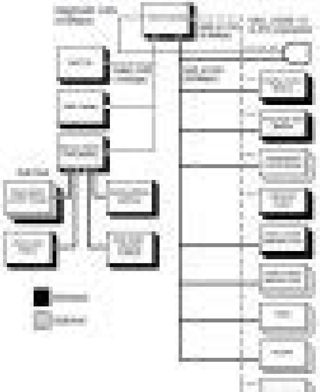
Figure 1: System Architecture
