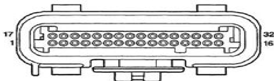
VCM Connector C1 (BLU)
