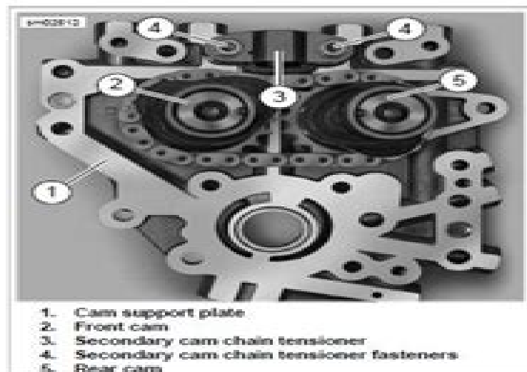
Figure 3-96. Camshafts
