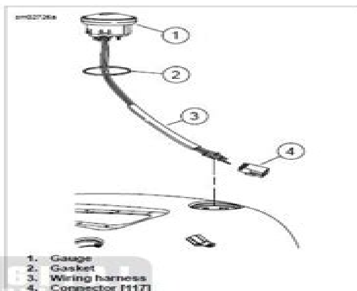
Figure 7-69. Fuel Gauge
