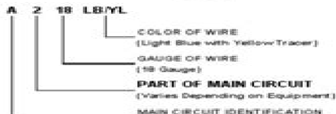
Figure 1 – Wire Color Code Identification
