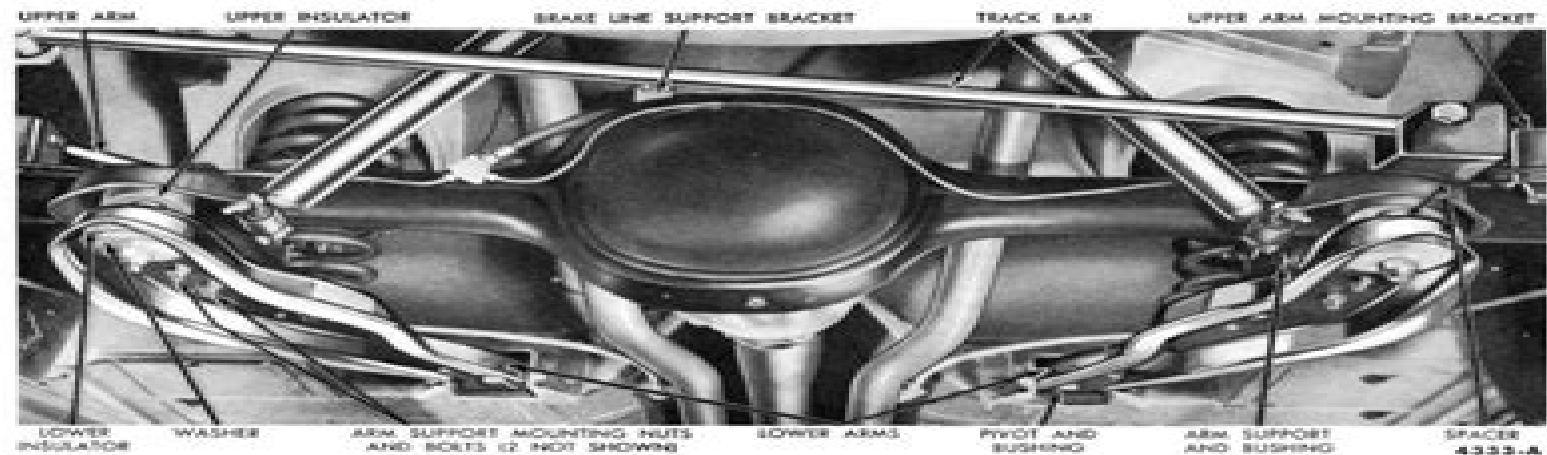
FIG. 14—Rear Suspension
