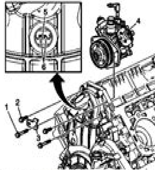
Fig. 112: Identifying Turbocharger Cooler Return Pipe Bracket & Bolts Courtesy of GENERAL MOTORS COMPANY
