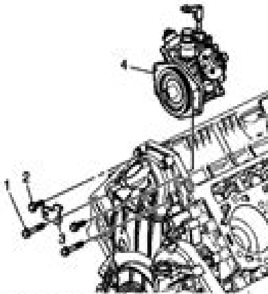
Fig. 111: View of Fuel Injection Pump & Bolts Courtesy of GENERAL MOTORS COMPANY
