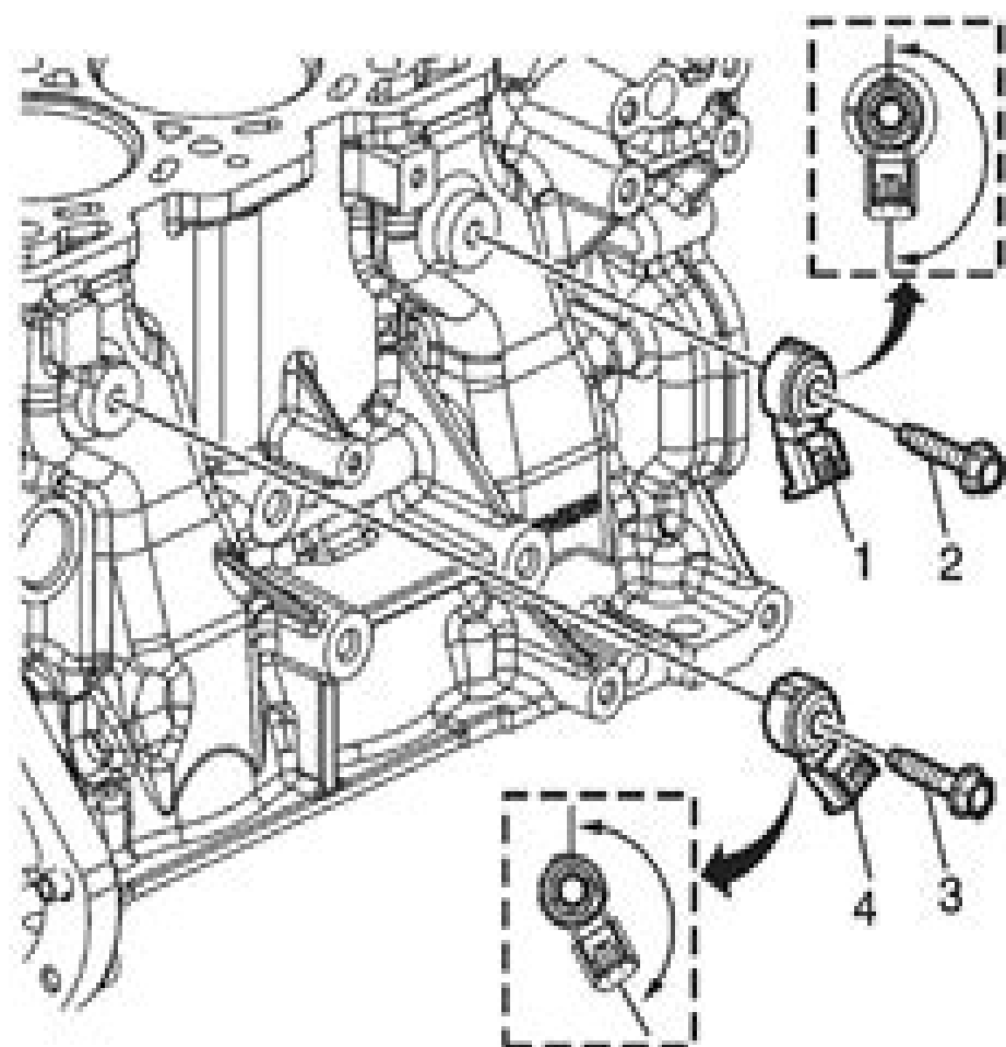
Fig. 213: Knock Sensor
