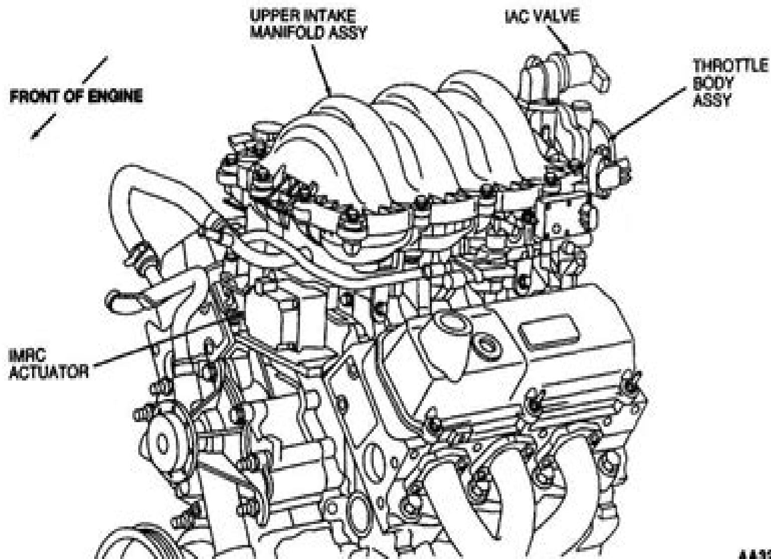
Figure 112: 3.8L Windstar Intake Air System
