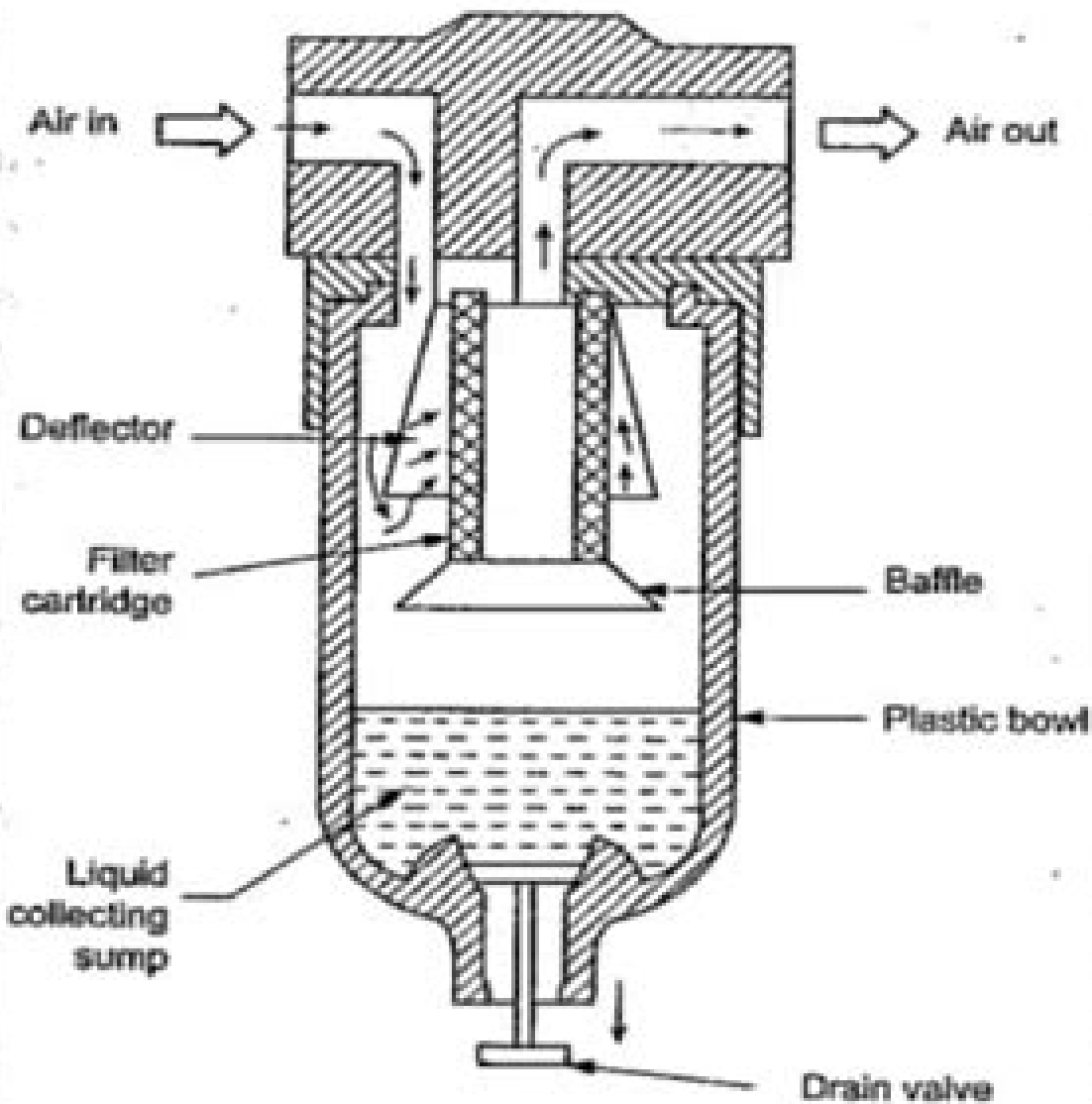
(a) Construction and operation
