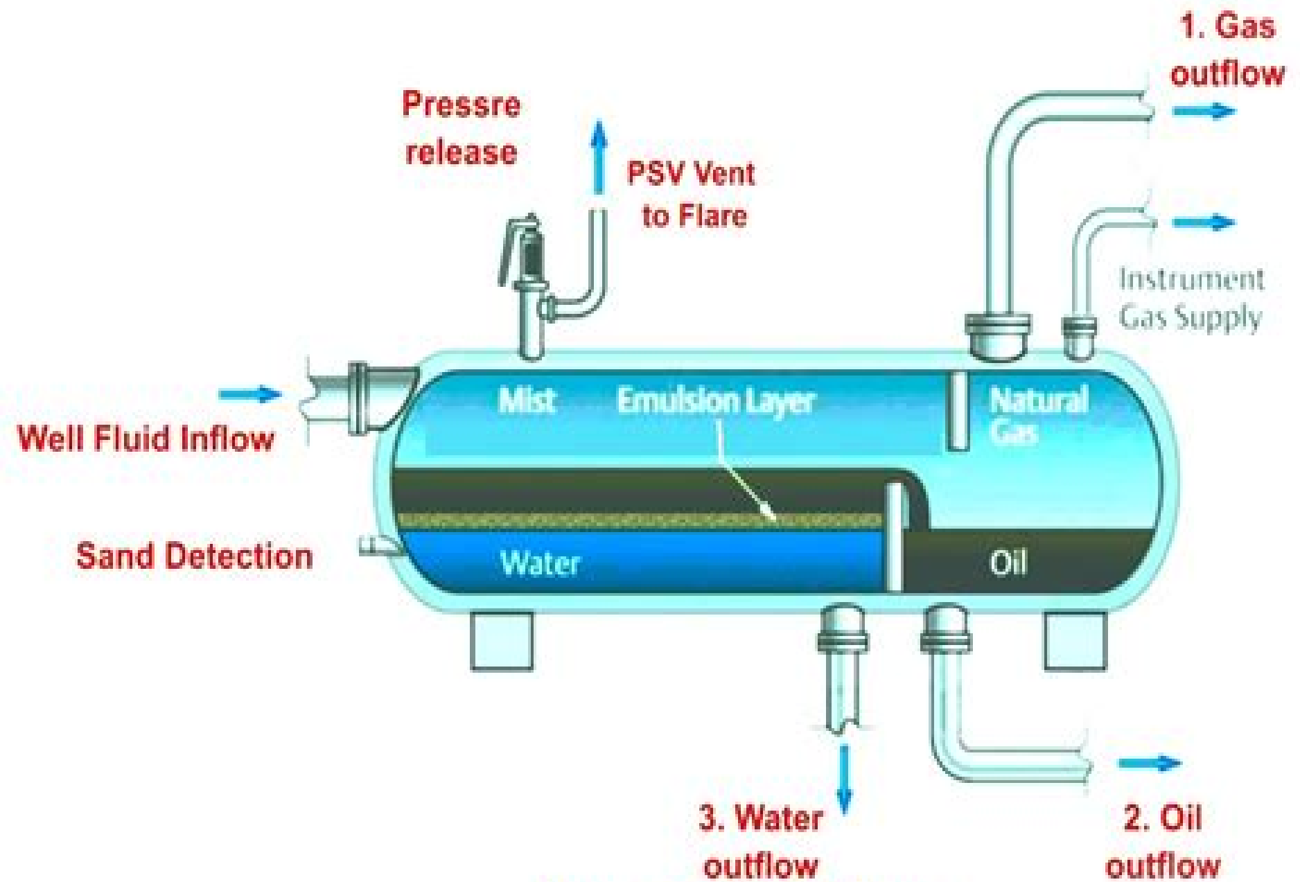
Process Separator 3 Phase
